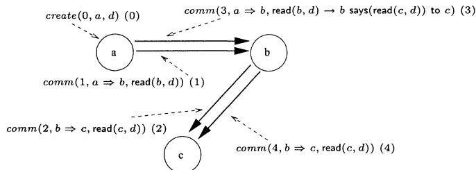
Figure 1. The actions of Alice (a), Bob (b) and Charlie (c) in our example. Solid arrowed lines represent communications, dashed lines represent observable events.
