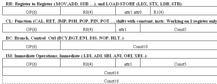
Figure 4. Instruction Formats
