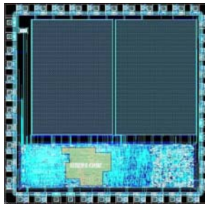
Figure 9. Prototype ePille- SOC-ASIC layout in 0.35 AMI CMOS technology, (not complete), Size is 11mm 2
