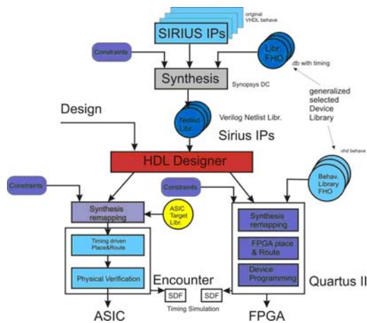
Figure 6. Netlist based IP development and dissemination
