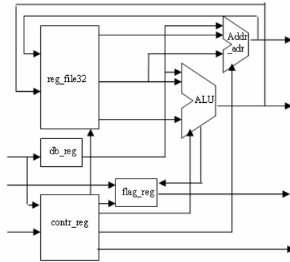
Figure 1. Block diagram of the SIRIUS soft core
