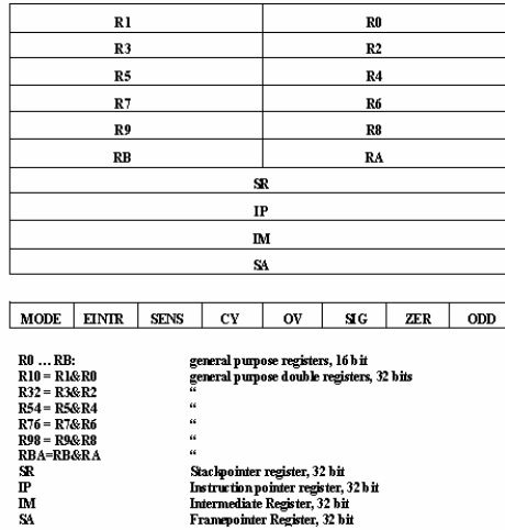
Figure 2. Programmer's Model
