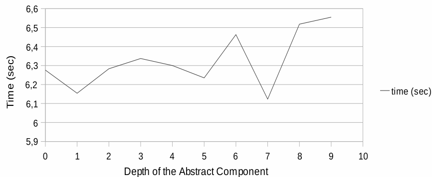
Fig. 5. The time for turning abstract primitive components into concrete ones.
