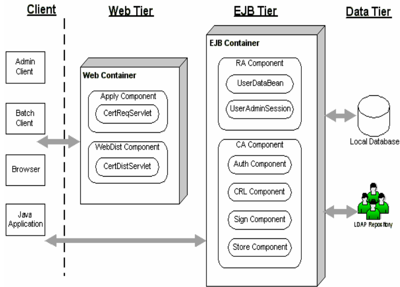
Fig. 1. System framework of EJBCA
