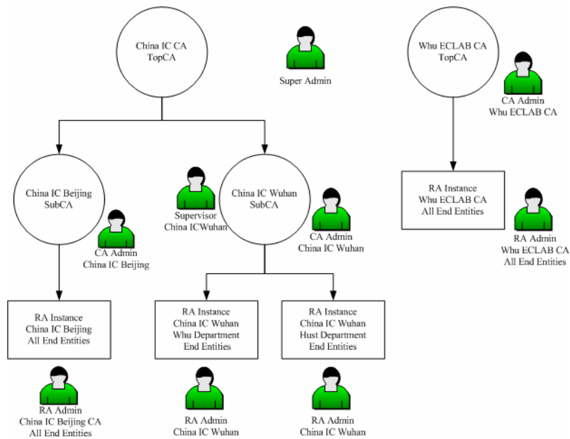
Fig. 3. The basic framework of the application
