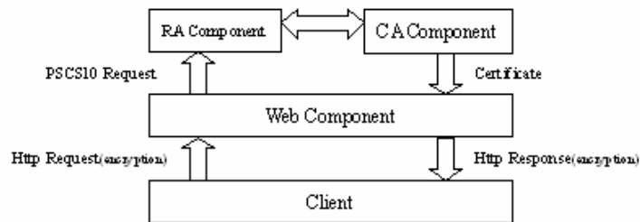
Fig. 2. The process of information transmission in EJBCA
