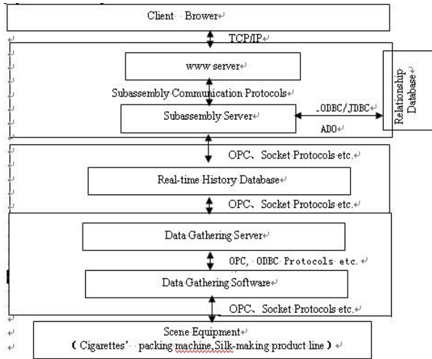
Figure. 4 MES Software Structure
