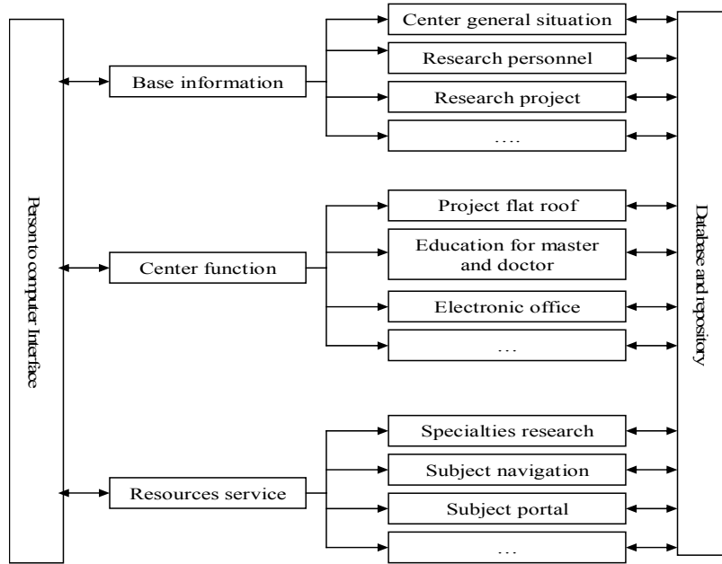
Fig. 2. Function frame of CSIR portal
