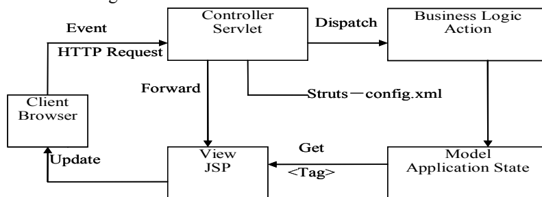
Fig. 4. MVC framework based on Struts
