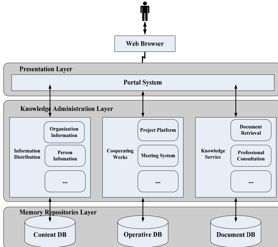
Fig. 1. Integrated system of information portal
