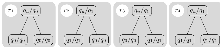
Fig. 2. The transition rules of the percolate protocol.
