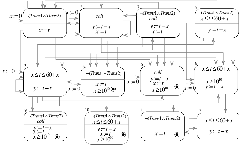
Fig. 4. The Optimized tableau automata of \Box_{[0,10^{10}]}\left((Trans1 \wedge Trans2) \rightarrow \diamond_{[0,60]}coll\right)
