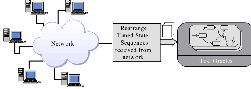
Fig. 2. The role of test oracle in software testing
