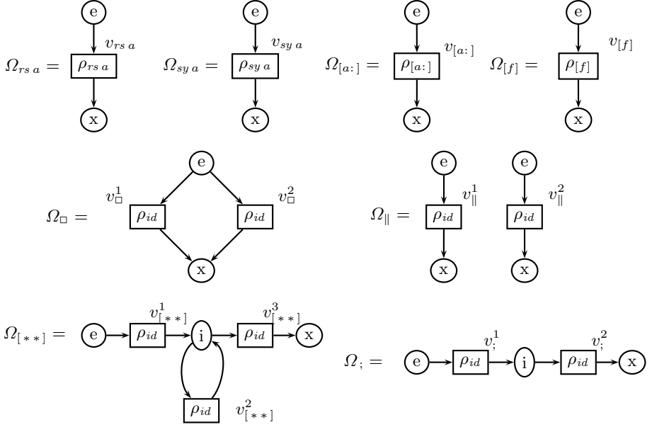
Fig. 1. The operator s-boxes for sPBC
