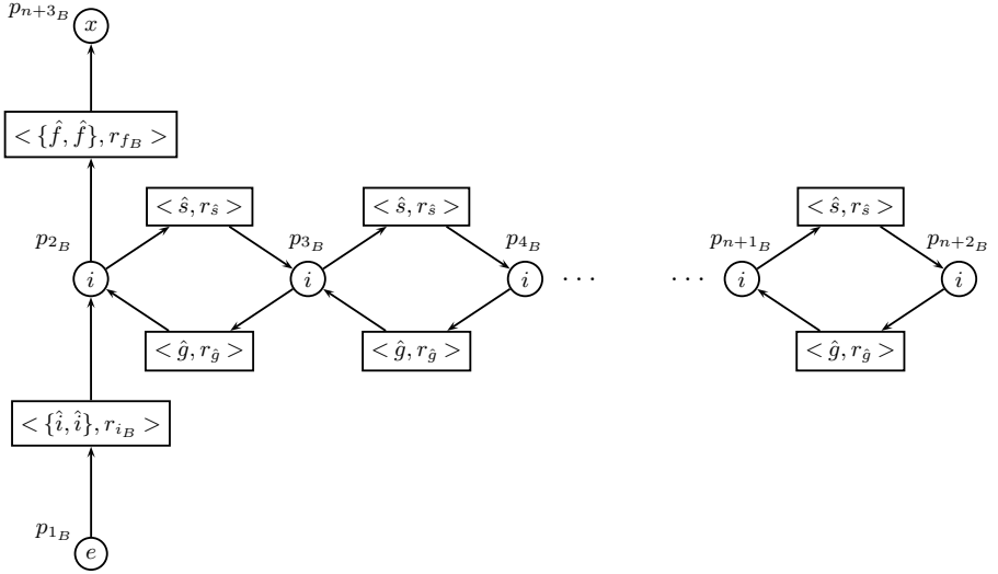
Fig. 2. Plain s-box of Buffer_n
