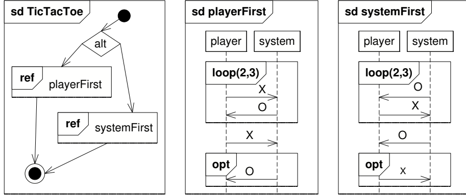
Fig. 1. Playing tic-tac-toe
