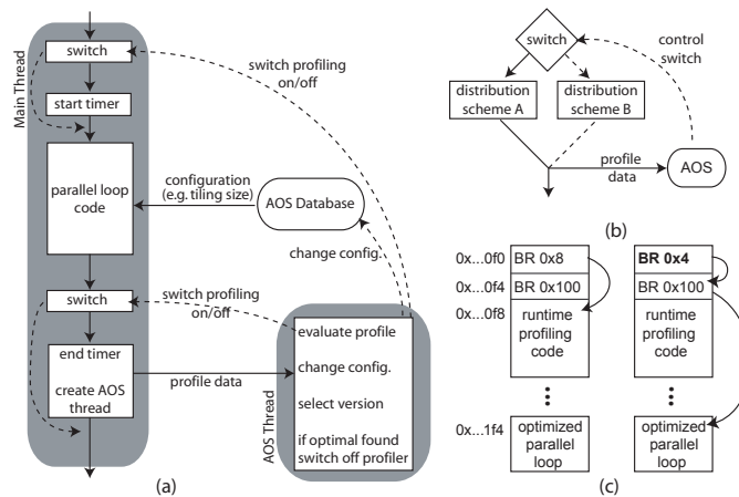
Fig. 1. Runtime profiling and adaptive version switching.
