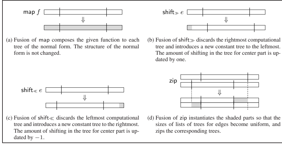
Fig. 1. An image of fusion rules. Rectangles show the resulting lists. The three parts separated by vertical lines correspond to the triple of a normal form. Changed parts are shaded.
