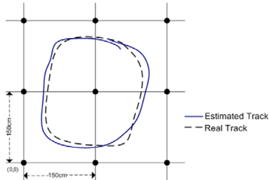
Fig. 7. Tracking the moving node
