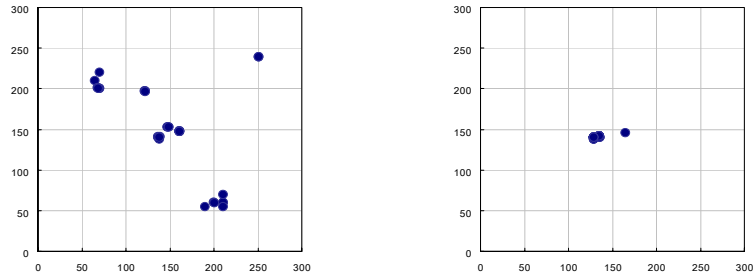
(c) Without error filtering and radio reliability: position (150,150) (d) Error filtering and radio reliability : position (150,150)
