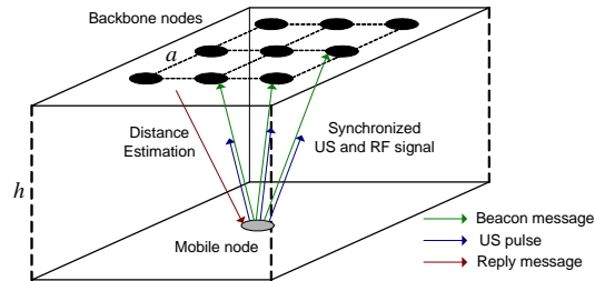
Fig. 1. Active tracking system
