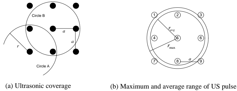
Fig. 5. Ultrasonic range
