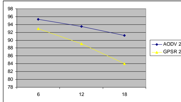
Fig. 1. Success Ratio versus Intensity.
