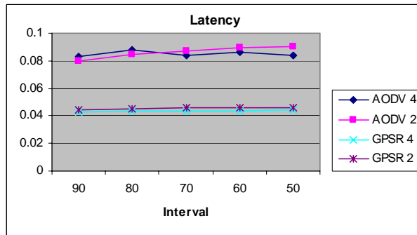
Fig. 4. Delay versus Interval.
