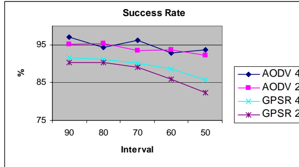
Fig. 3. Success Ratio versus Interval.
