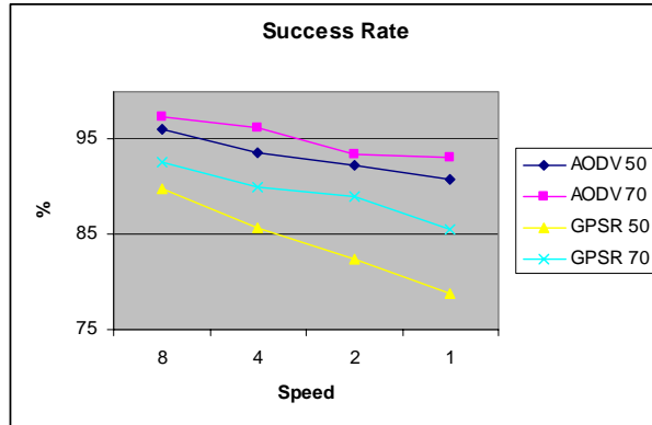
Fig. 5. Success Ratio versus Speed.
