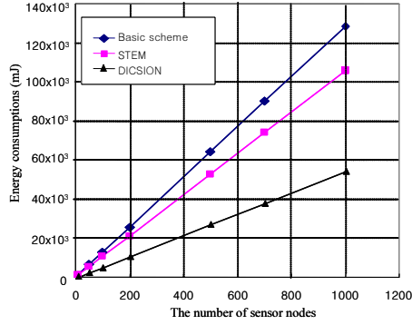
Fig. 6. Theoretical result.
