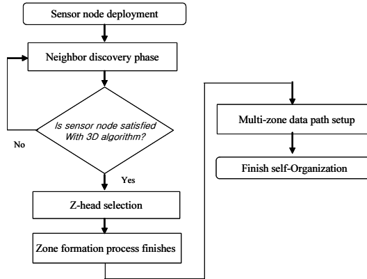
Fig. 3. The zone formation algorithm of DICSION.
