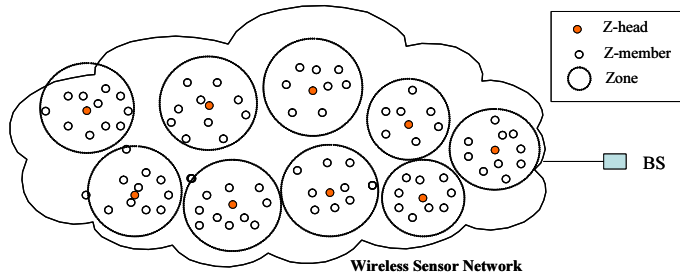
Fig. 2. DICISION architecture.
