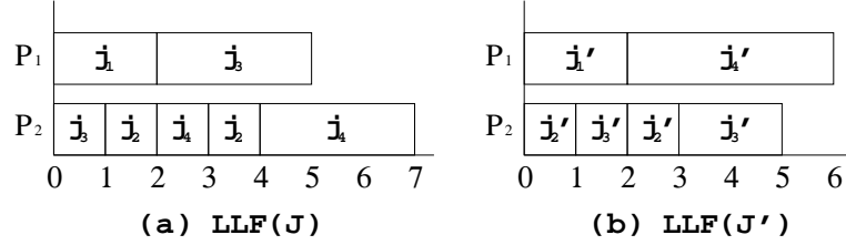
Fig. 1. LLF is not start time predictable if the actual execution time is known.
