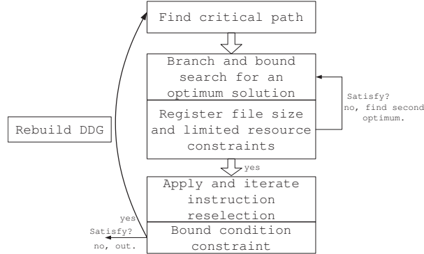
Fig. 2. Algorithm overview
