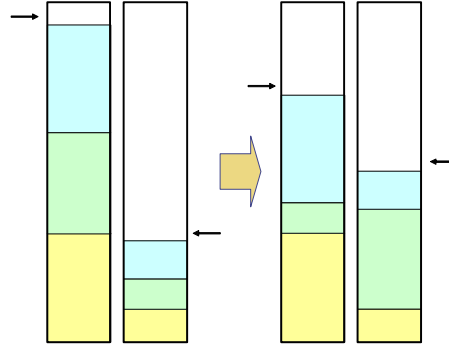
Fig. 2. Balanced dual run-time environment
