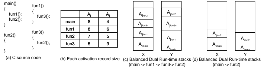
Fig. 3. Example of balanced dual run-time stacks
