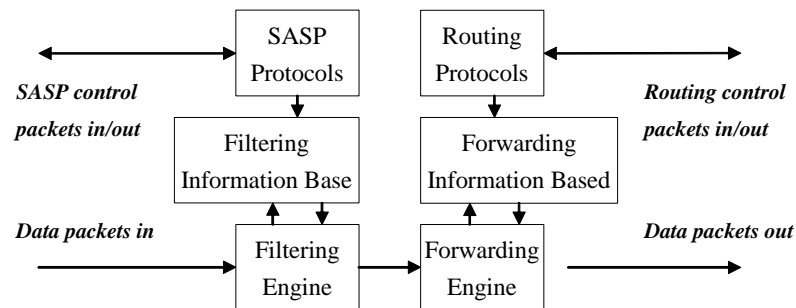
Fig. 3. Architecture of the SASP router
