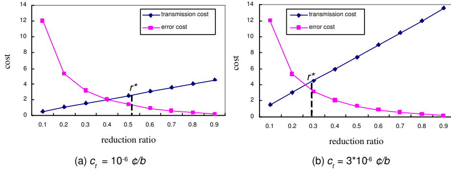
Fig. 4. Cost Trade-off for the 2-level Caching Structure ( b_0 = 10 \text{Kb/s} , c_e = 1 \phi / \% , N_0 = 500 , k = 2 , q_0 = 10 , q_1 = 20 )
