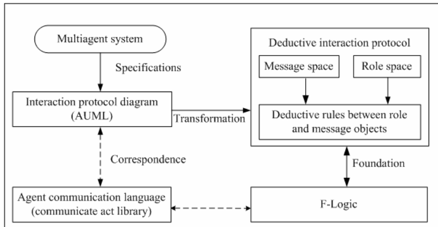
Fig. 1. The AUML/F-logic transformation framework
