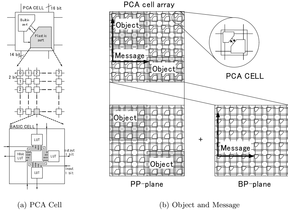
Fig. 1. Plastic Cell Architecture
