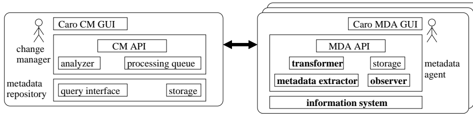
Fig. 1. Caro architecture
