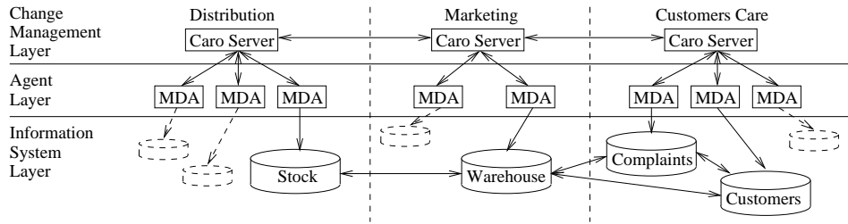
Fig. 2. Distributed Caro architecture
