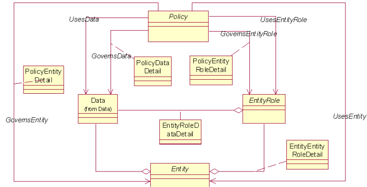
Fig. 3. Overall model of policy, data, entity and role (subclasses omitted for readability)
