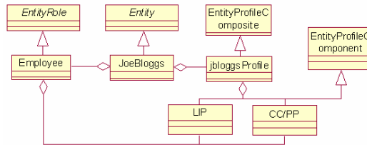
Fig. 2. – Example of Entity JoeBlogs with role Employee, profile and profile components.
