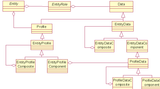
Fig. 1. – The Data model
