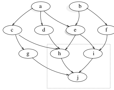
Fig. 2: Random scheduling of precedence constrained policies.
