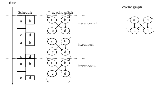
Fig. 5: Keeping schedules of iterations disjoint to ensure no intra cycle dependency violations.
