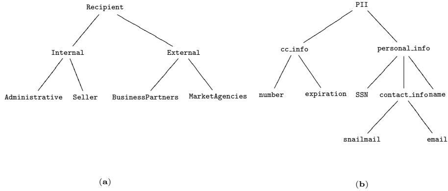
Fig. 1. An example of recipient hierarchy (a) and data type hierarchy (b)
