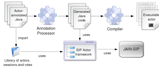
Fig. 5. Coding framework architecture
