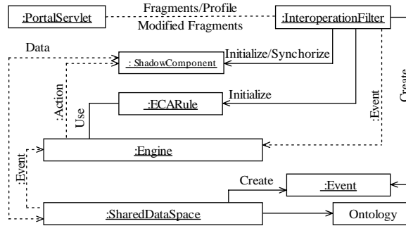
Fig. 6. Collaboration Diagram of Portlet Interoperation
