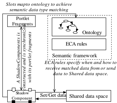
Fig. 4. Portlet interoperation model
