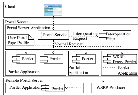
Fig. 5. Portlet interoperation process
