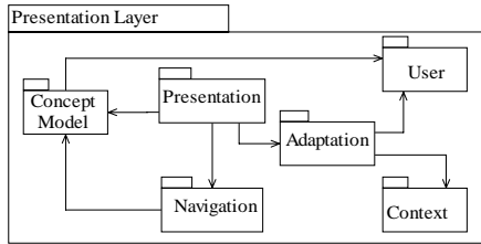
Fig. 3.(a) Presentation model of a portlet
