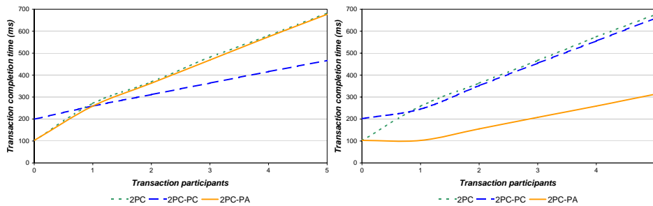
Fig. 5. High commit rate.
