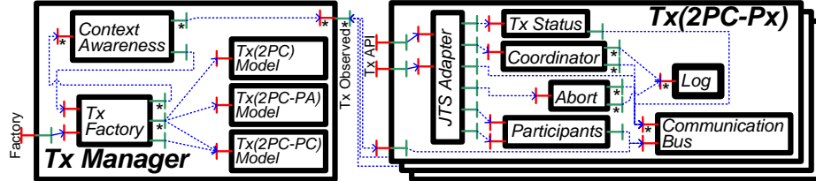
Fig. 8. CATE component-based architecture.
