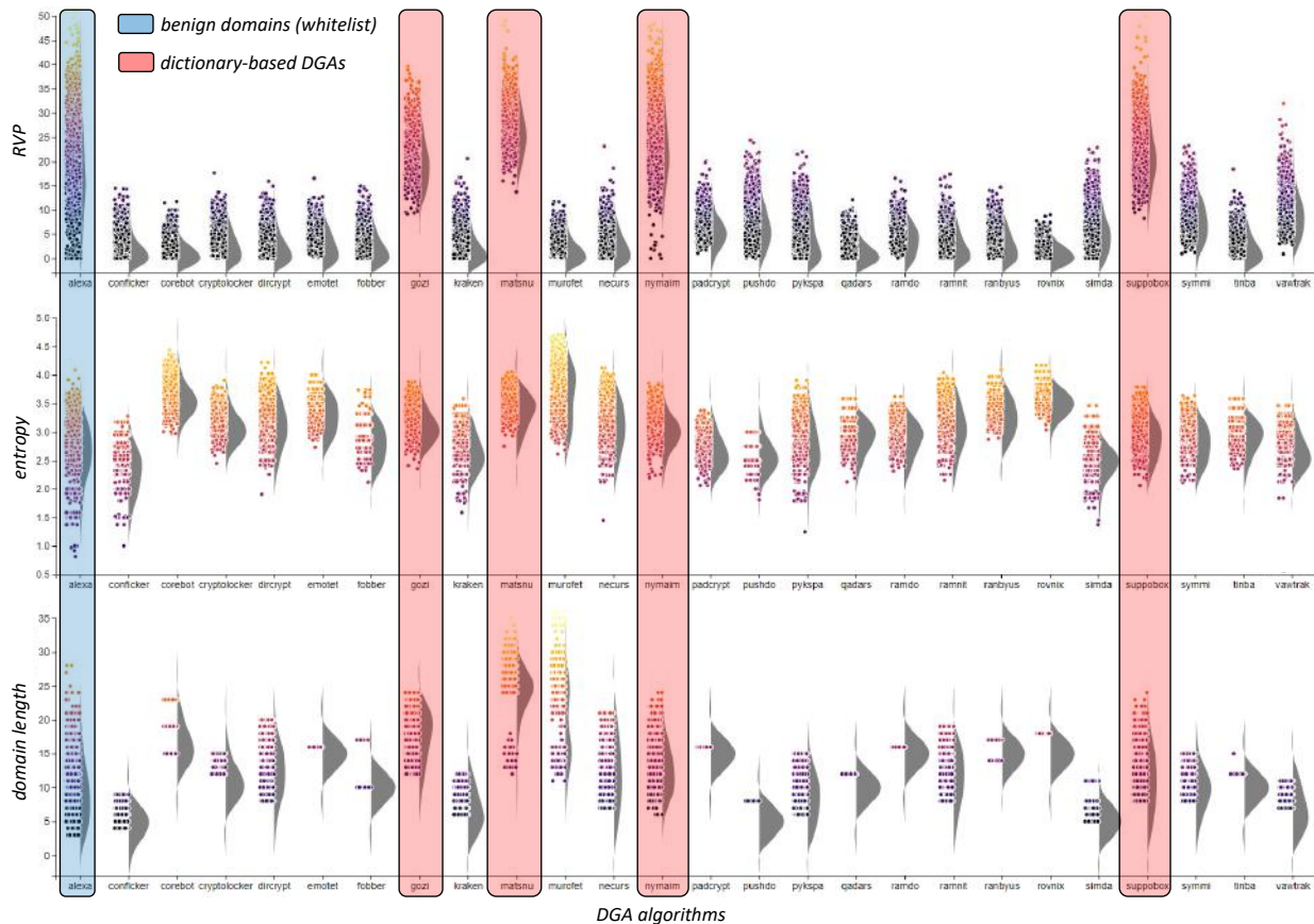
Figure 3. Empirical distribution of the input features used by RF3, for benign domains (alexia) and per DGA type. For ease of comparison, dictionary-based DGA algorithms are marked with boxes. DGAs such as emotet, padcrypt, or pushdo generate domains of constant length.
