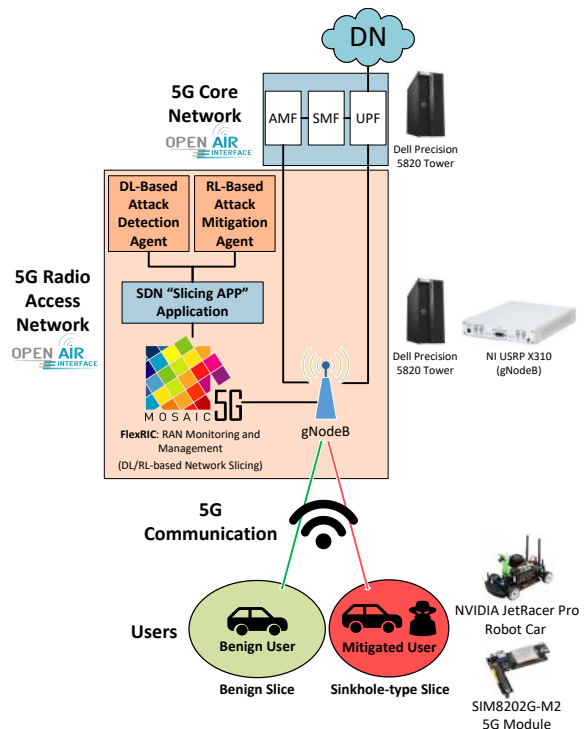
Fig. 1: 5G-V2X testbed's base hardware/software resources.
