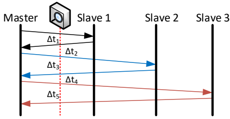
Fig. 2. Master-oriented traffic profiles.
