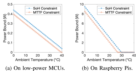
Fig. 5: P_{SoH} and P_{MTTF} regarding different devices.
