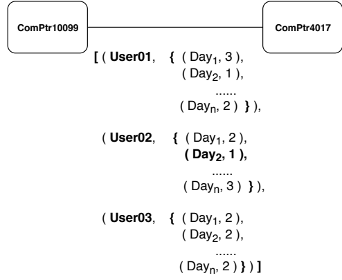
Fig. 2. Graph representation of authentication events
