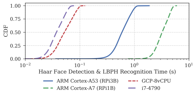
Fig. 1. Overall computation time for 640 \times 460 PNG on different hardware: a Raspberry Pi 1B, a Raspberry Pi 3, a Google Cloud Platform VM and a server CPU (Intel i7-4790) with a GPU (GeForce GTX 950).
