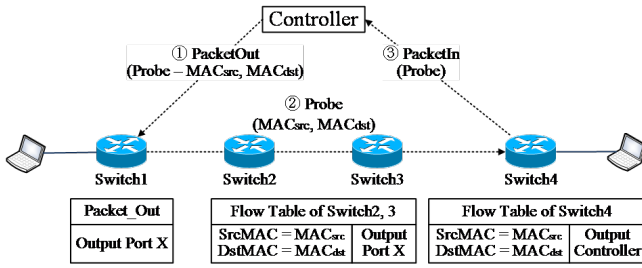
Fig. 1. Example of Probe-based Measurement
