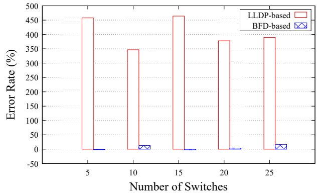
Fig. 7. Single Link Latency Error Rate (%)
