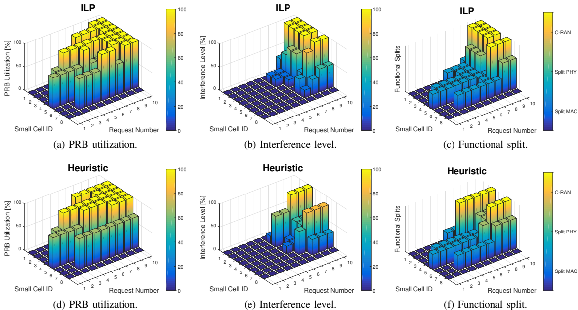
Fig. 5: PRB utilization, interference level and functional splits of the ILP-based and the heuristic algorithms.
