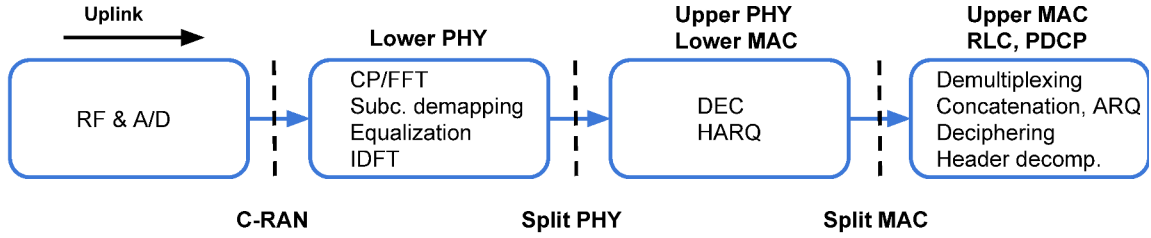
Fig. 1: Signal processing along with some of the functional split options within the RAN protocol stack in LTE networks.
