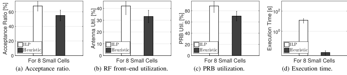
Fig. 3: Acceptance ratio, RF front-end and PRB utilizations, and the execution time of the ILP and the heuristic algorithms.
