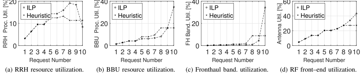
Fig. 4: Resource utilization using both the ILP and the heuristic placement algorithms.
