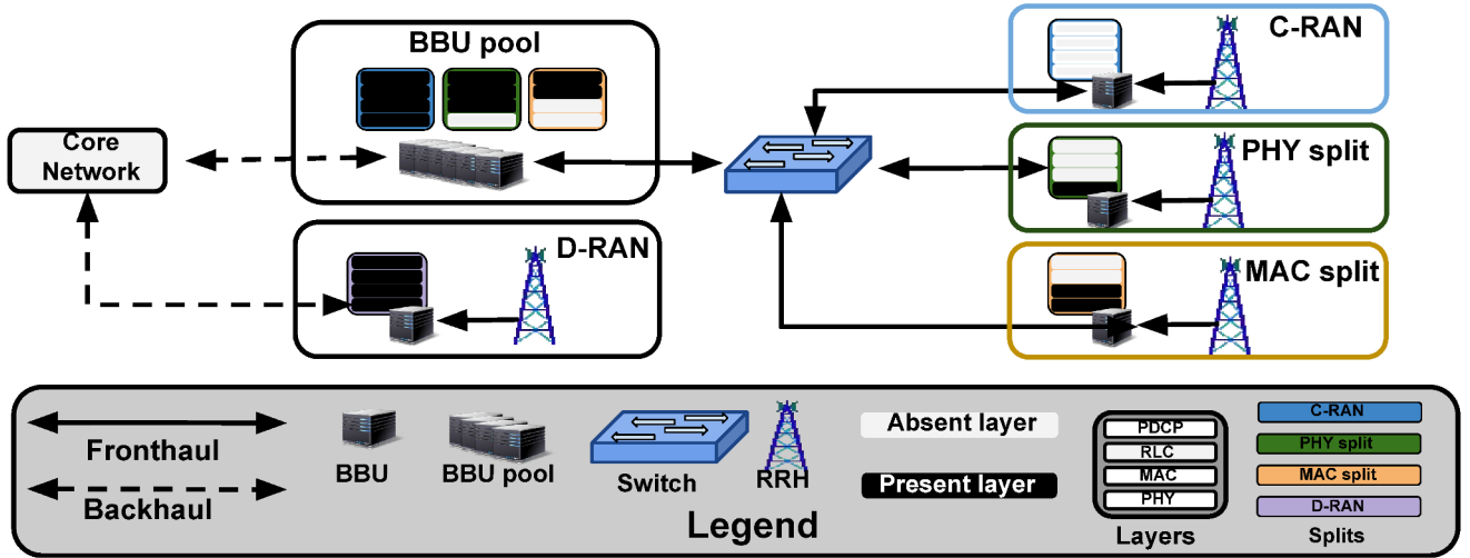
Fig. 2: The different functional splits that can co-exist at the BBU pool. Notice that, in the cases of the PHY and MAC splits, also the RRHs possess processing capabilities.
