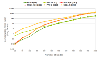
Fig. 4: Computation Time
