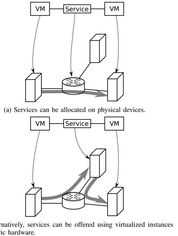
Fig. 2: NFV service chain allocation approaches.
