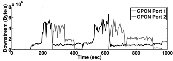
(a) Downstream traffic at the GPON ports
