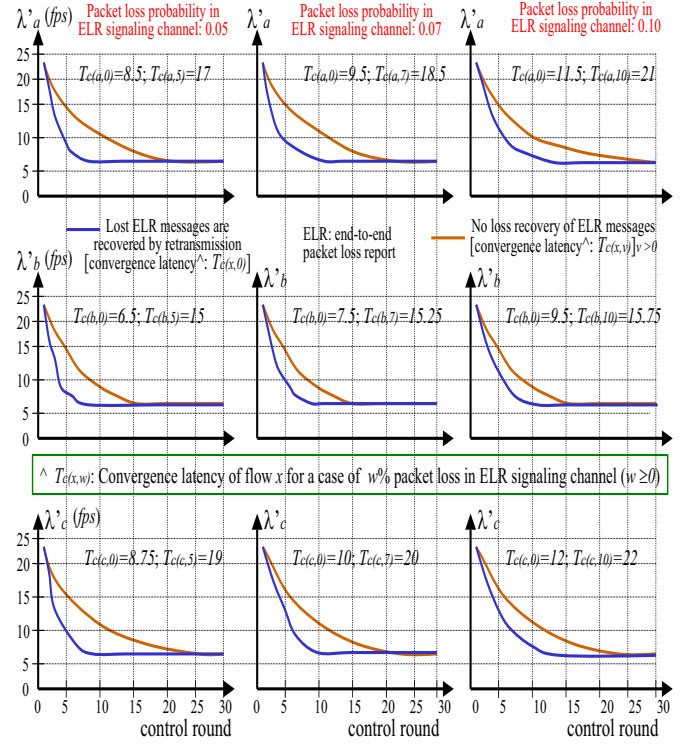
Fig. 6. Impact of ELR signaling errors on convergence behavior of sources
