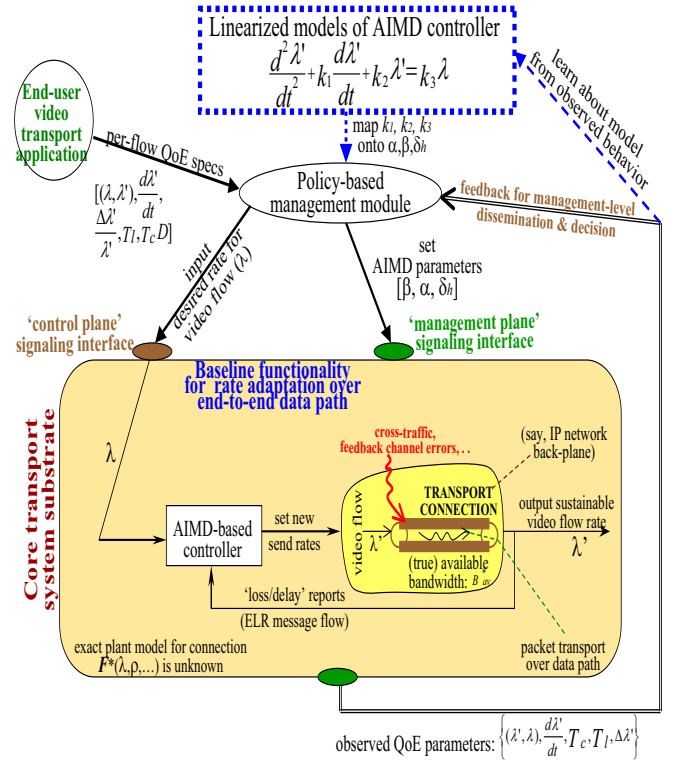
Fig. 5. Model-based supervision of rate adaptation in BAVT system
