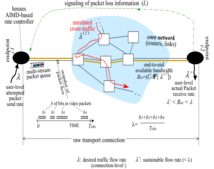
Rate-adaptive video transport system over a bandwidth-limited network
