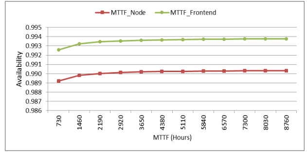
Figure 4: Effect of failure times on system availability.
