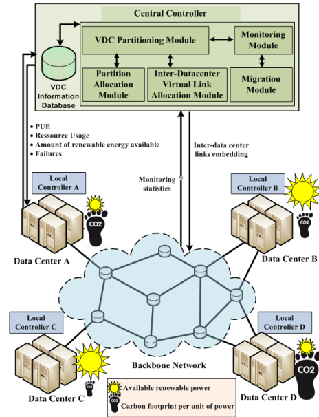
Fig. 1: Proposed framework
