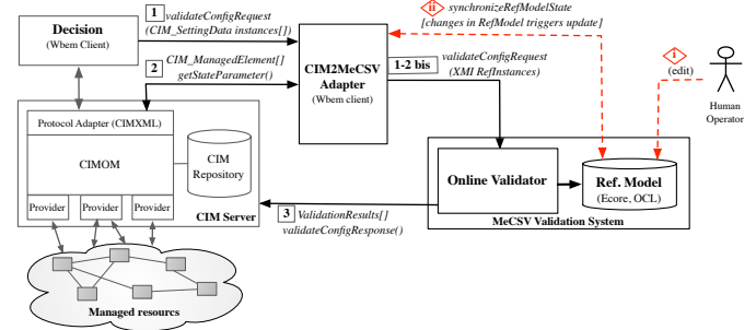
Fig. 3. Integration with CIM/WBEM: runtime architecture
