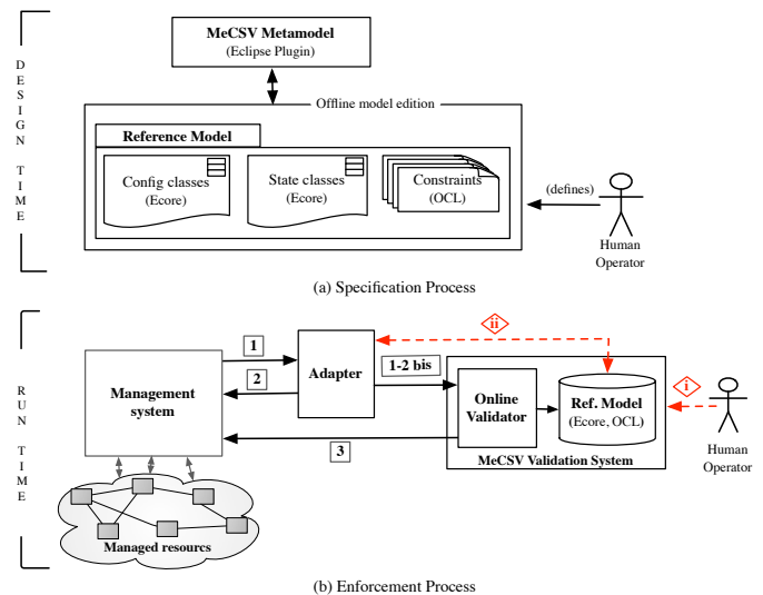
Fig. 2. Framework's Approach and Runtime Architecture
