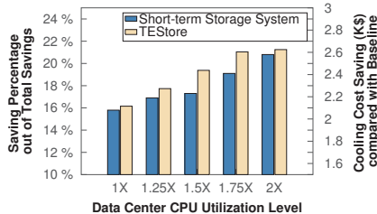
Fig. 5. Cooling cost savings and saving distributions of TEstore under different utilization levels.
