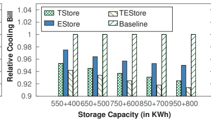
Fig. 9. Cooling cost comparison among different different storage strategies, under a series of different storage capacities.
