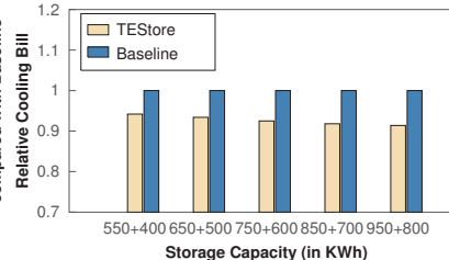
Fig. 6. Cooling cost savings of TEstore under different storage capacities.
