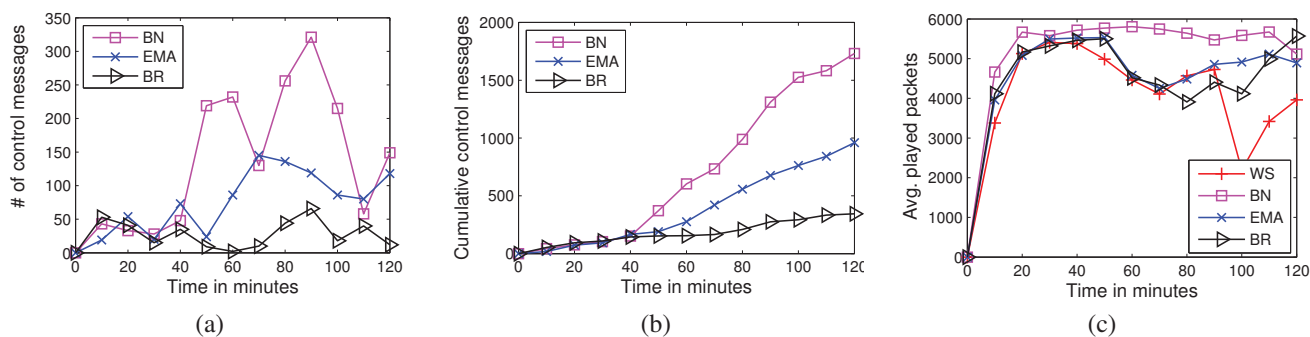
Fig. 4. (a) Control messages over a 10 minutes slot, (b) Cumulative control messages, (c) Packets meeting the playback deadline
