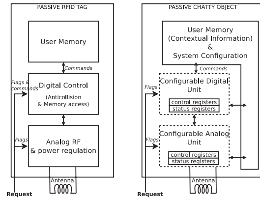
Fig. 2: Here are two simplified diagram block. On the left is a common RFID tag design. Its communication is driven by the flags field of the request and by others few specific commands. On the right, the behavior of a chatty object is configurable from the reader by accessing internal register or configuring programmable units.
