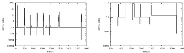
Fig. 12. Rates computed on layer 0 and 3 by Algorithm 2 on the data flow from R_8 to R_{11} .
