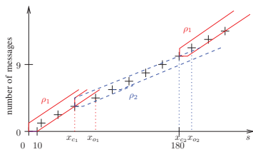
Fig. 2. Example of rates computed with Algorithm 2.
