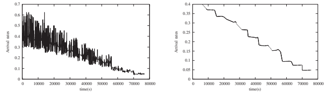
Fig. 7. Layer 0 and 3 of Algorithm 2 for a slowing down data flow.
