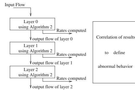
Fig. 4. Example of Algorithm 2 used with several layers.
