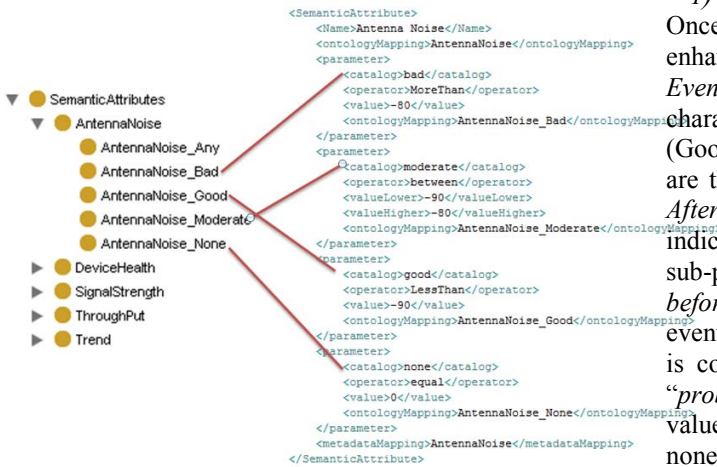
Figure 1. The mapping between Semantic Attributes and domain ontologies
