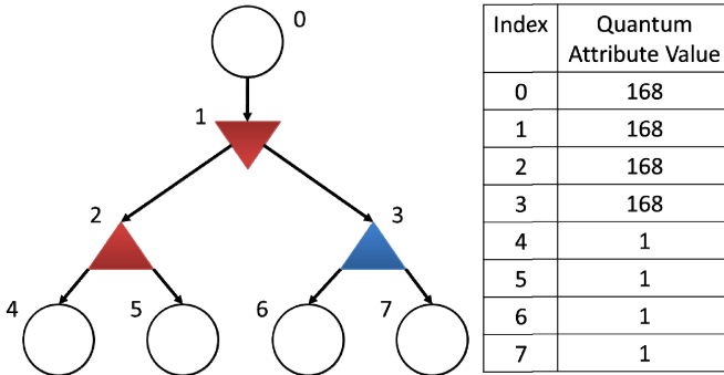
Figure 1: The Strategy Tree Used for Evaluation
